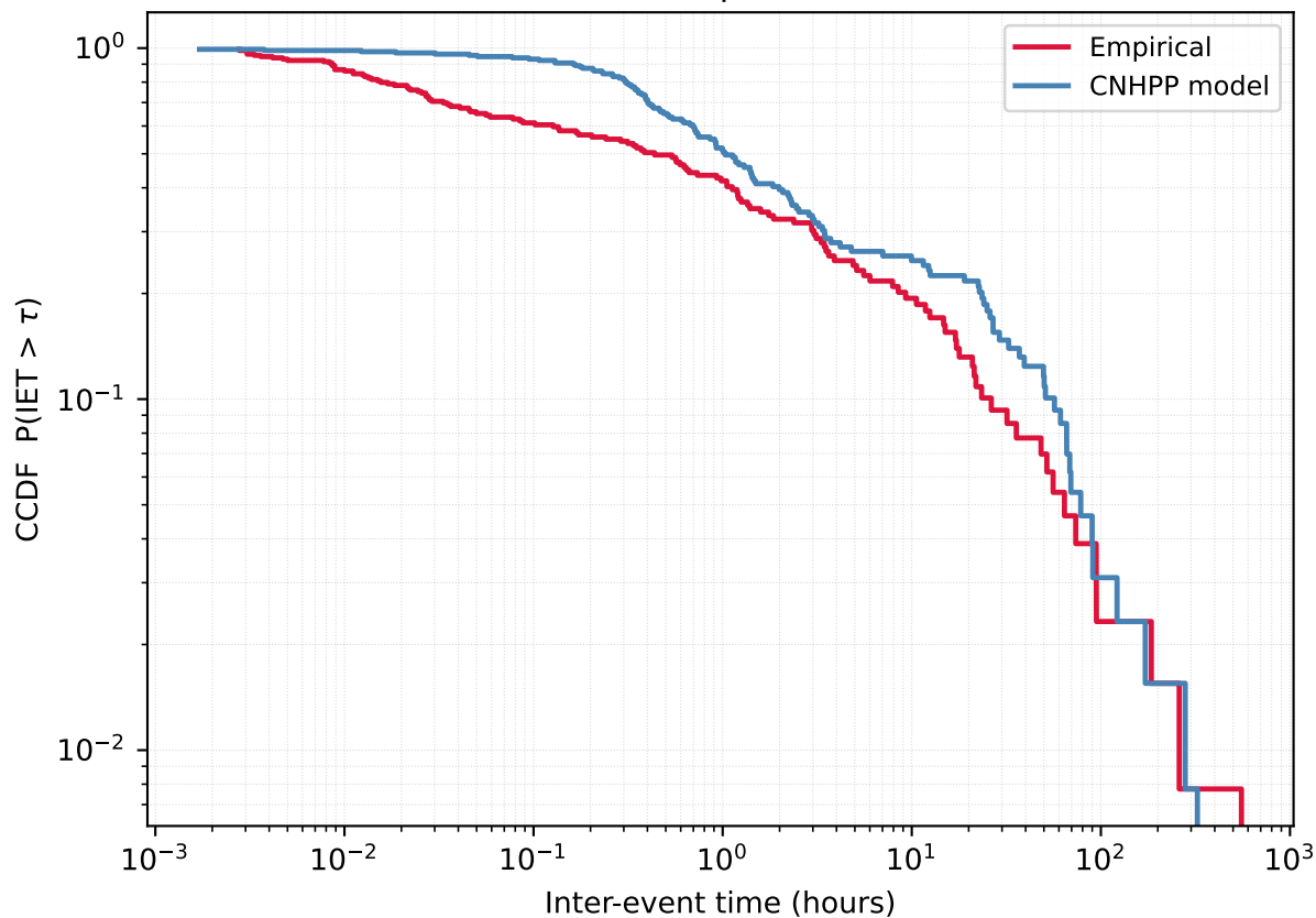
User 1889882810 - Empirical vs CNHPP model
